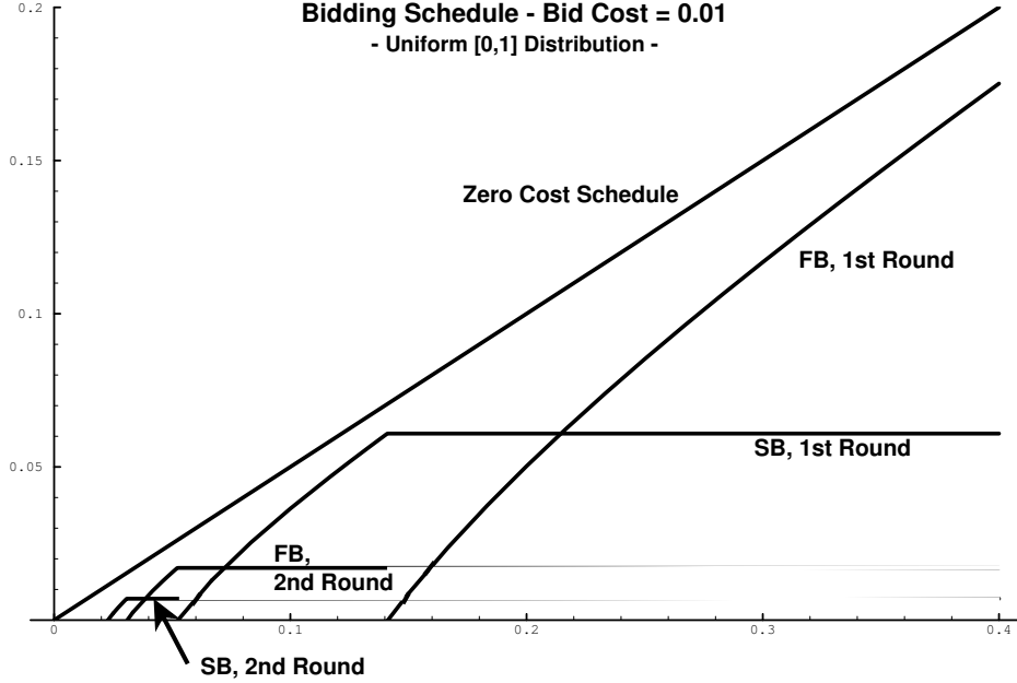
Fig. 1. First Four Bidding Schedules, Uniform [0, 1] Example, \gamma = 0.01
