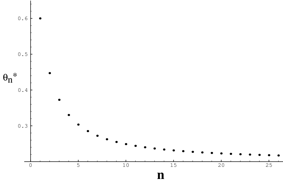
Fig. 2. Bidding Critical Value Sequence, n = 1, 26 .
